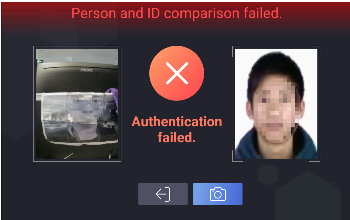
Figure 7-6 Failed Authentication
